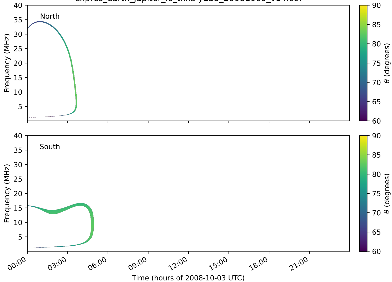
expres_earth_jupiter_io_txka-y235_20081003_v14.cdf
