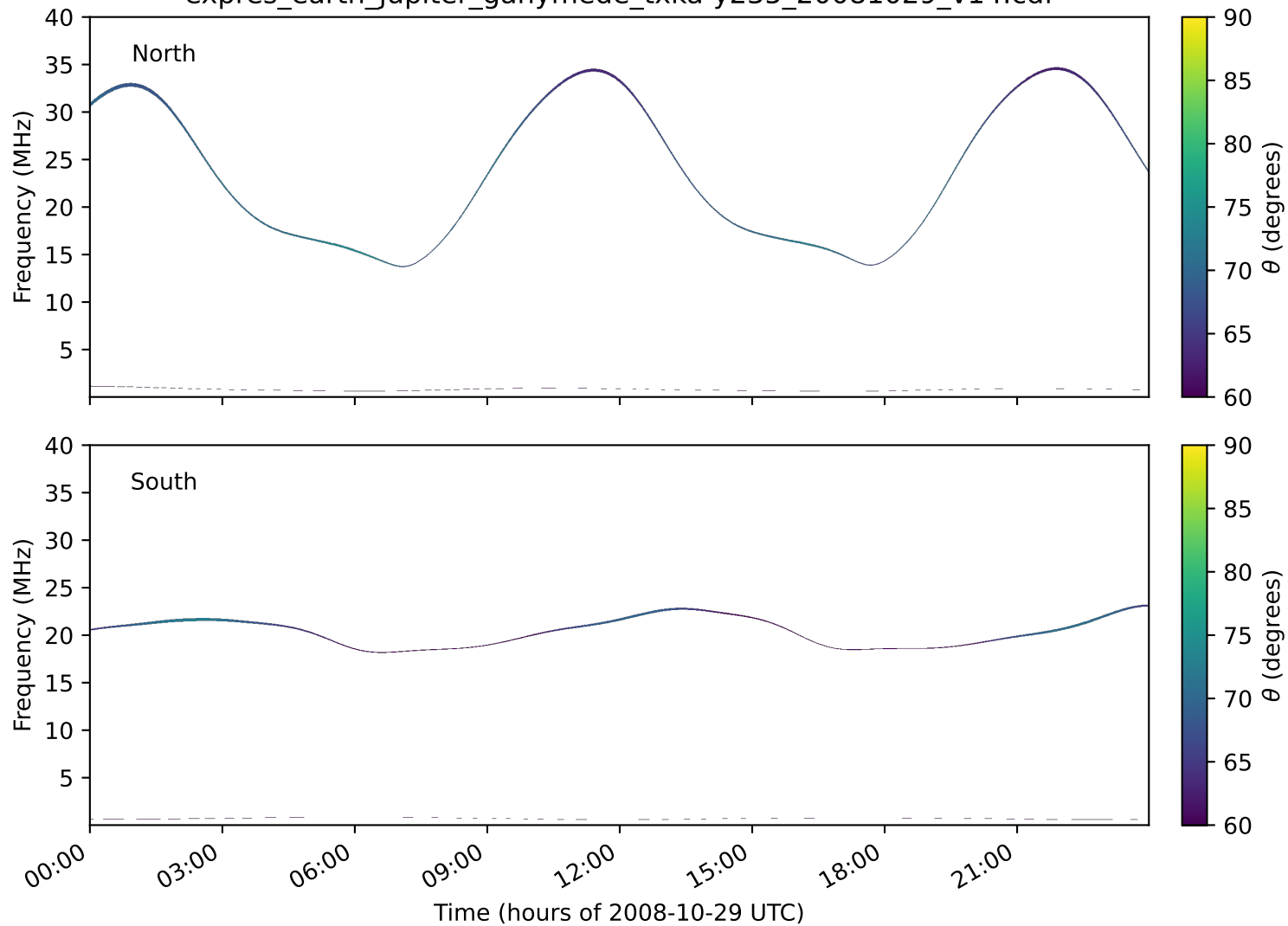
expres_earth_jupiter_ganymede_txka-y235_20081029_v14.cdf
