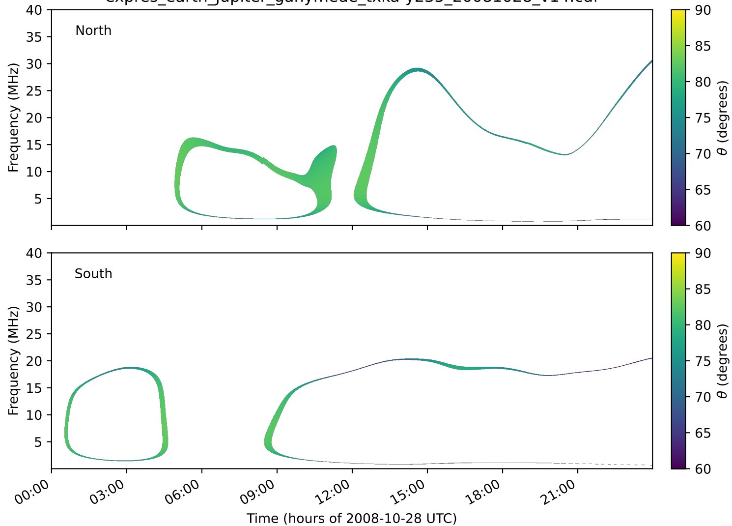
expres_earth_jupiter_ganymede_txka-y235_20081028_v14.cdf
