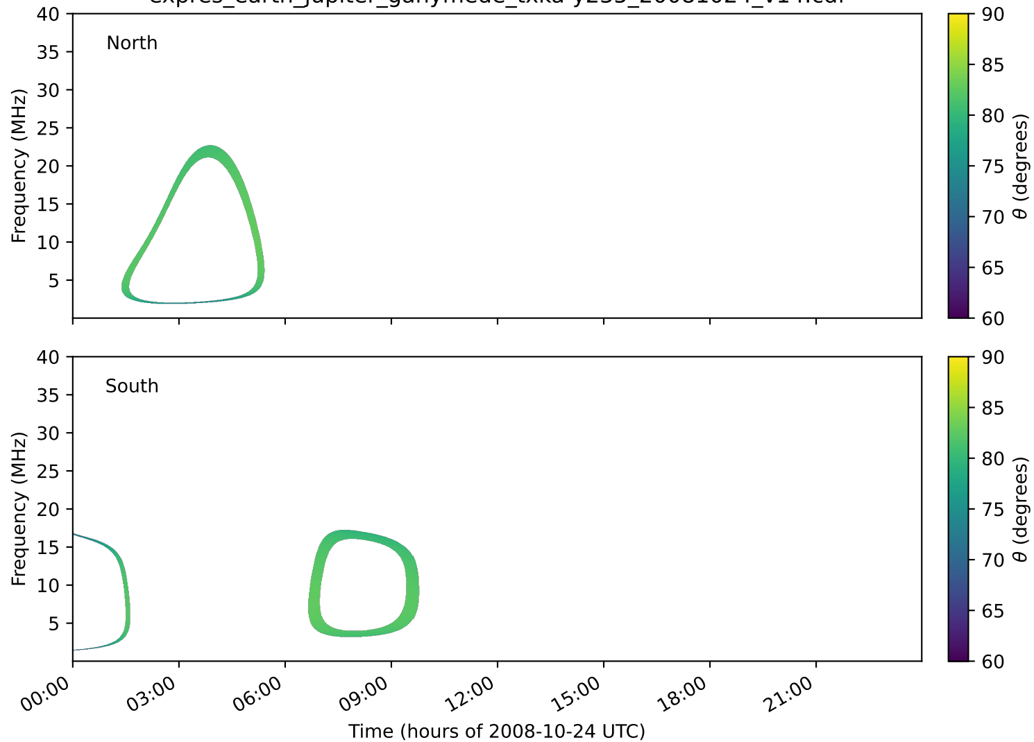
expres_earth_jupiter_ganymede_txka-y235_20081024_v14.cdf
