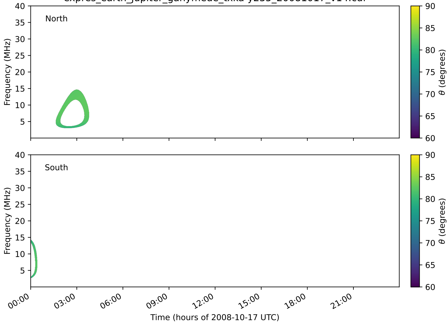
expres_earth_jupiter_ganymede_txka-y235_20081017_v14.cdf
