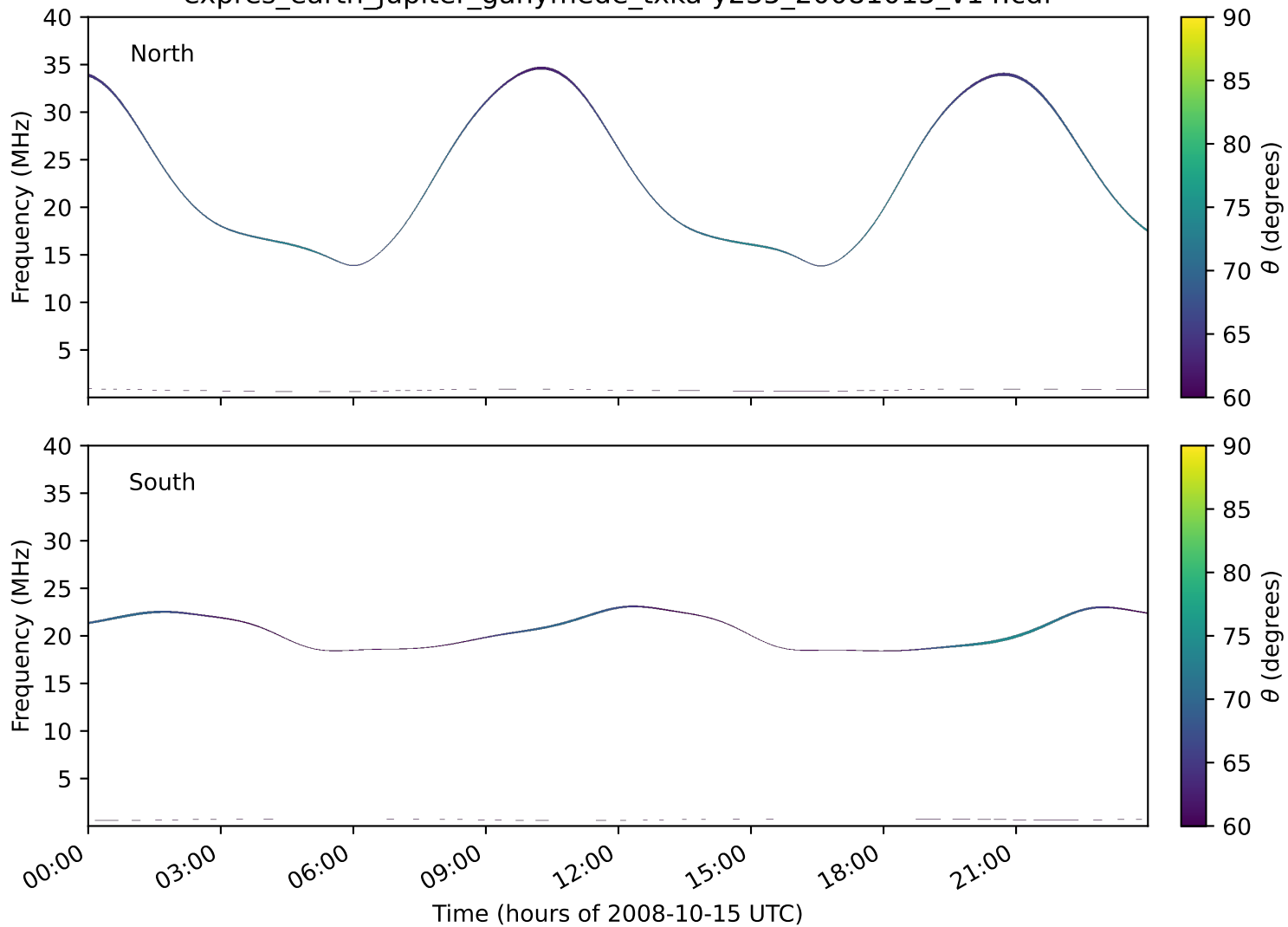
expres_earth_jupiter_ganymede_txka-y235_20081015_v14.cdf
