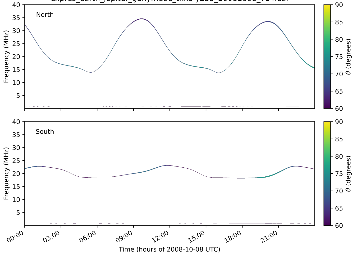
expres_earth_jupiter_ganymede_txka-y235_20081008_v14.cdf
