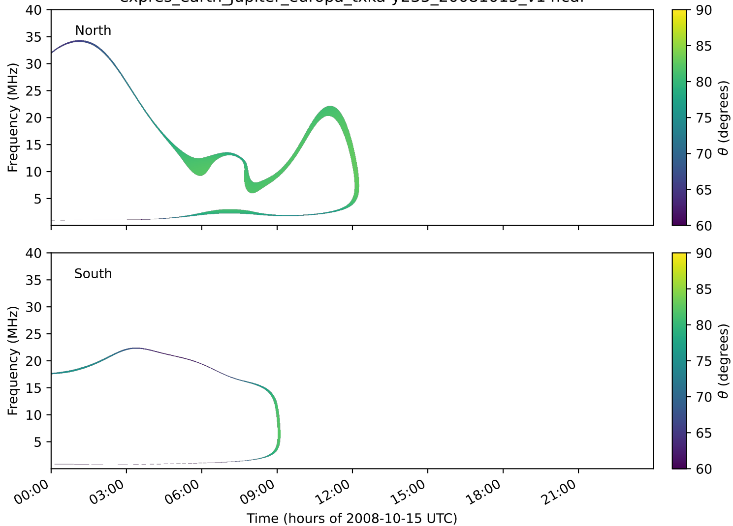
expres_earth_jupiter_europa_txka-y235_20081015_v14.cdf
