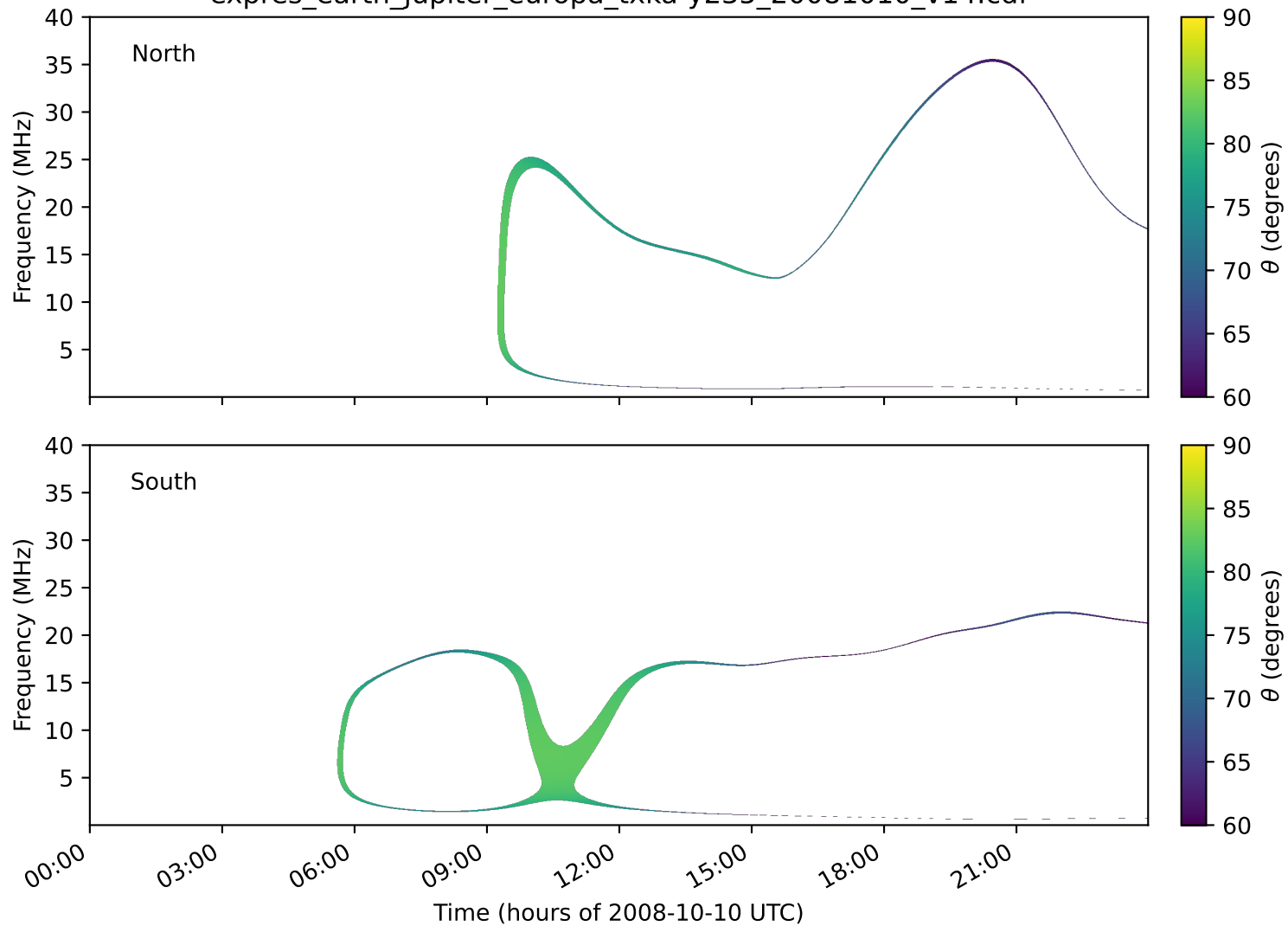
expres_earth_jupiter_europa_txka-y235_20081010_v14.cdf
