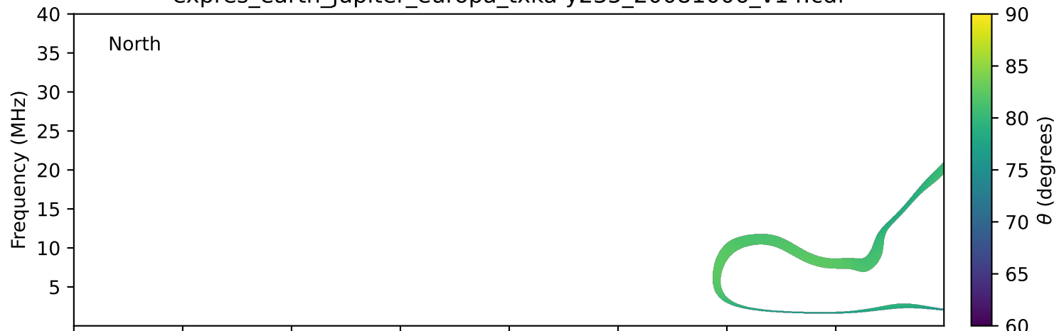
expres_earth_jupiter_europa_txka-y235_20081006_v14.cdf
