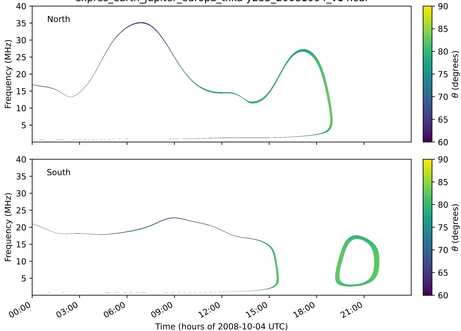
expres_earth_jupiter_europa_txka-y235_20081004_v14.cdf
