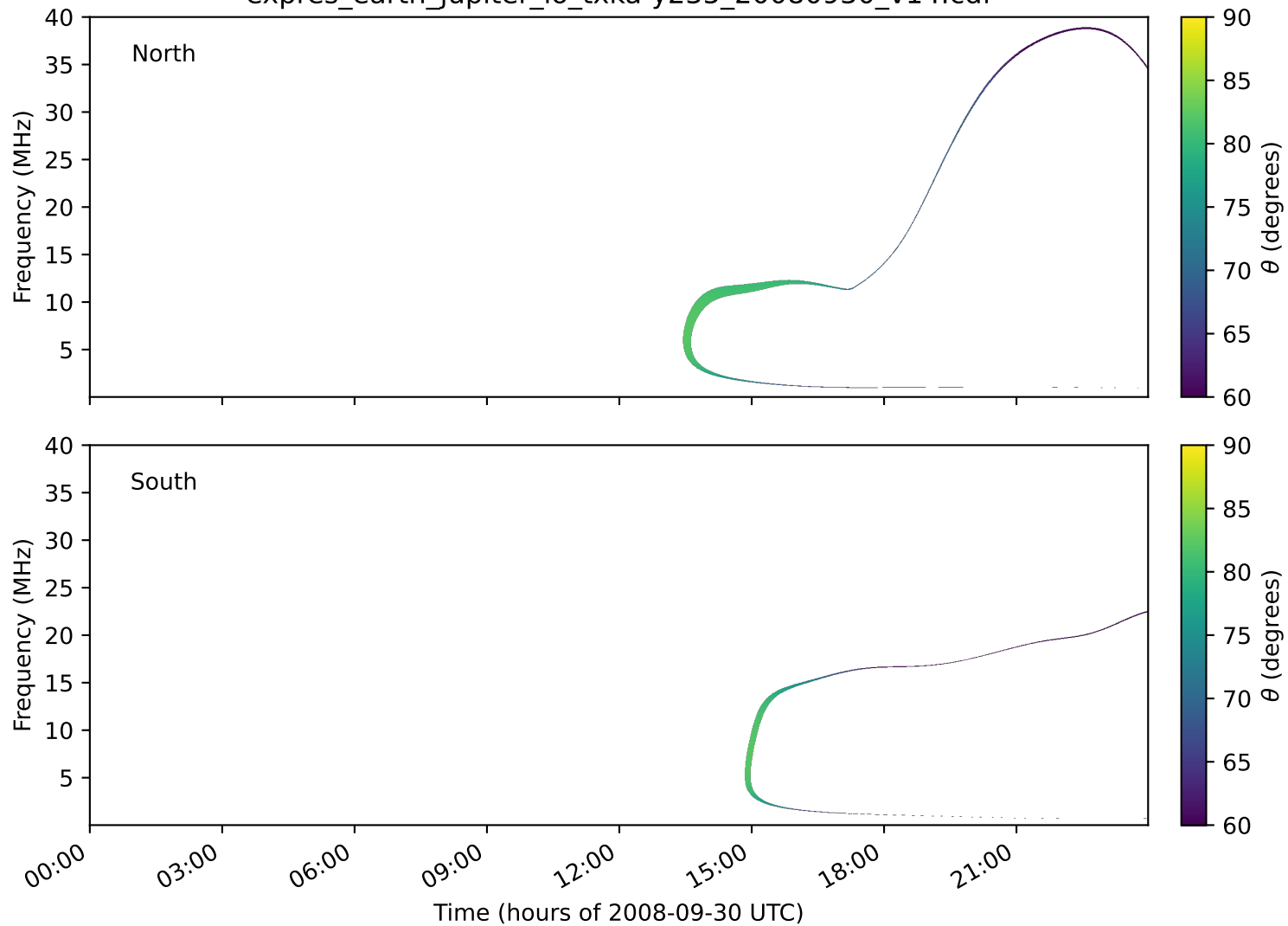
expres_earth_jupiter_io_txka-y235_20080930_v14.cdf
