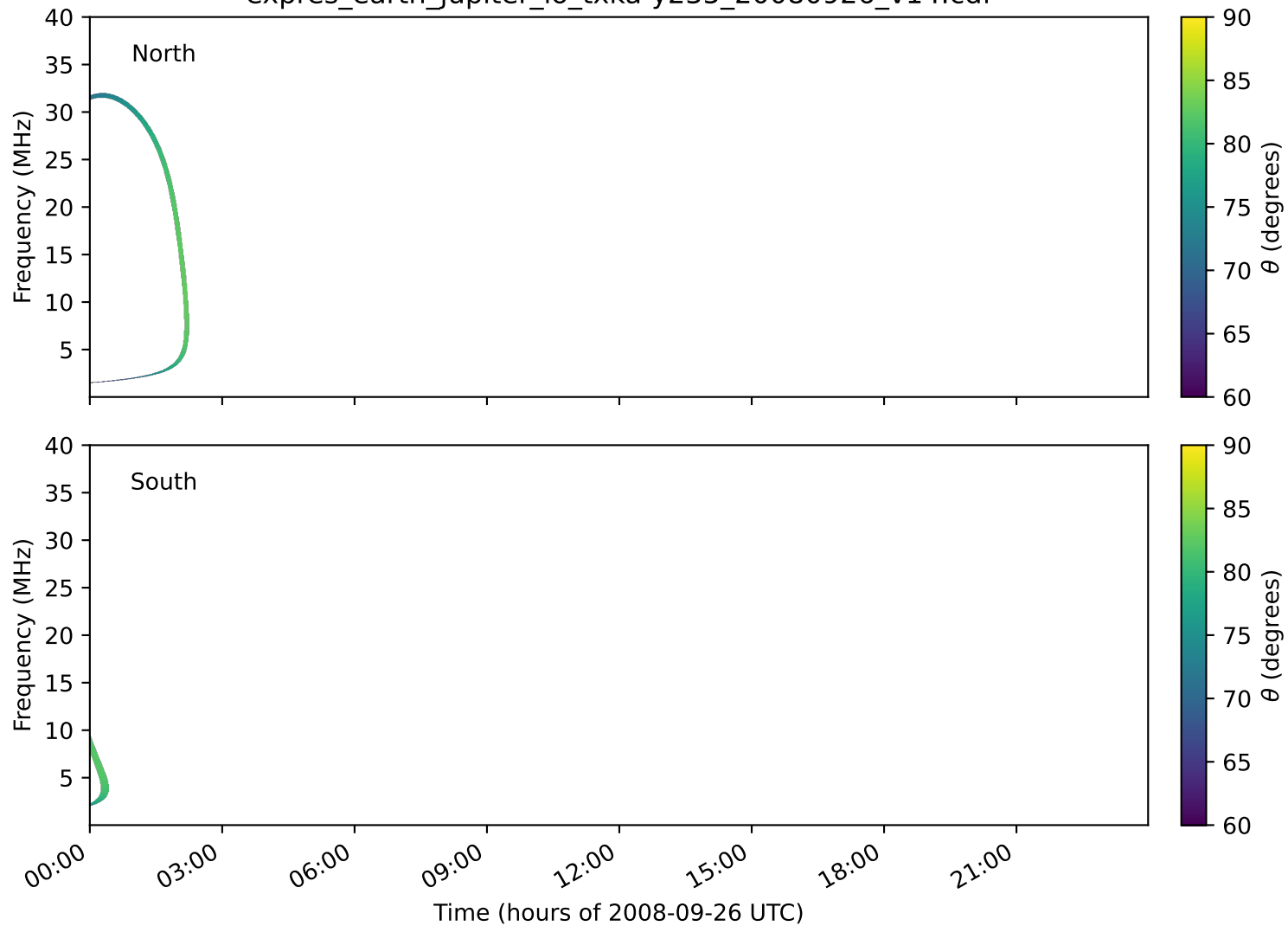
expres_earth_jupiter_io_txka-y235_20080926_v14.cdf
