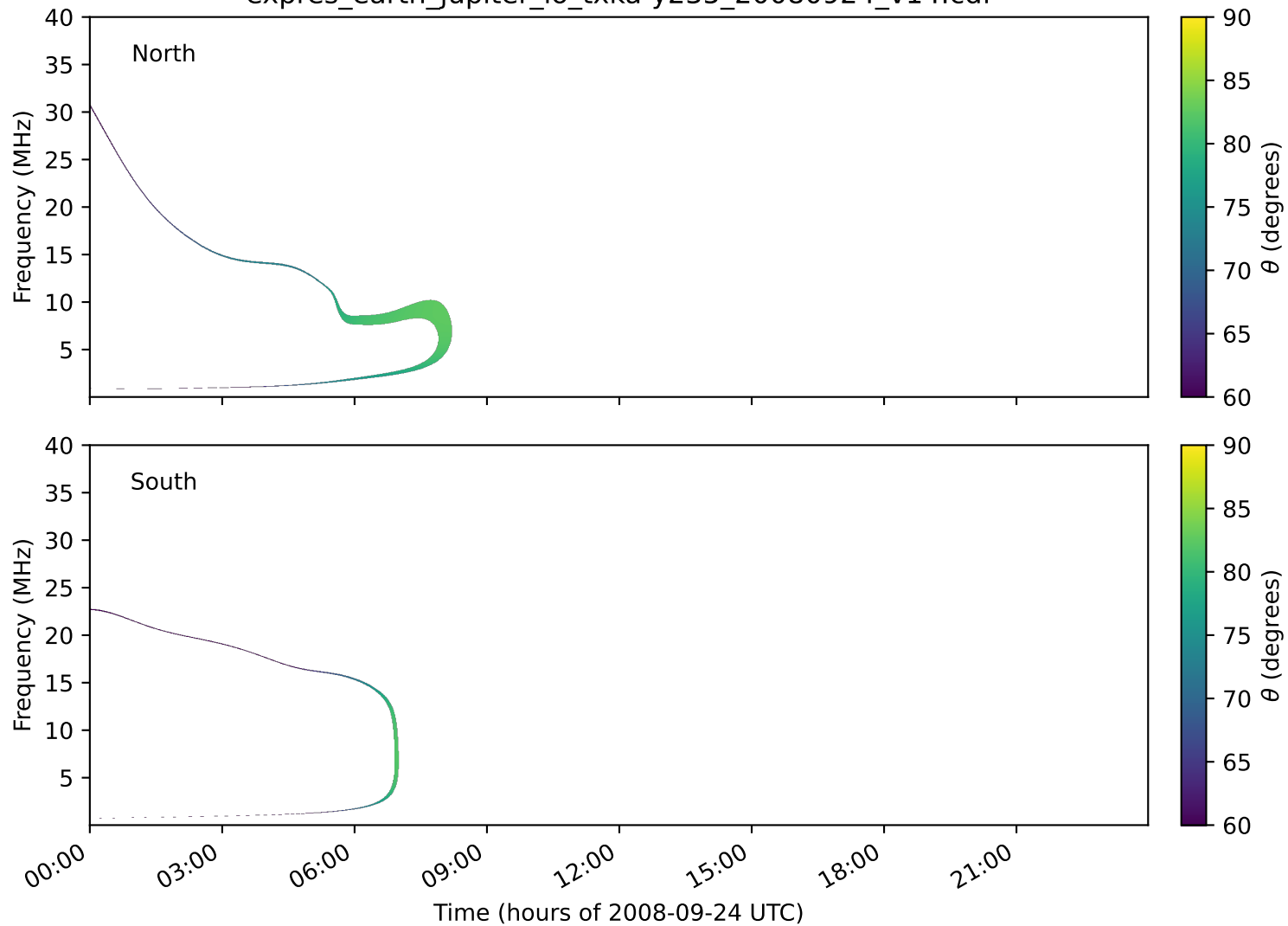
expres_earth_jupiter_io_txka-y235_20080924_v14.cdf
