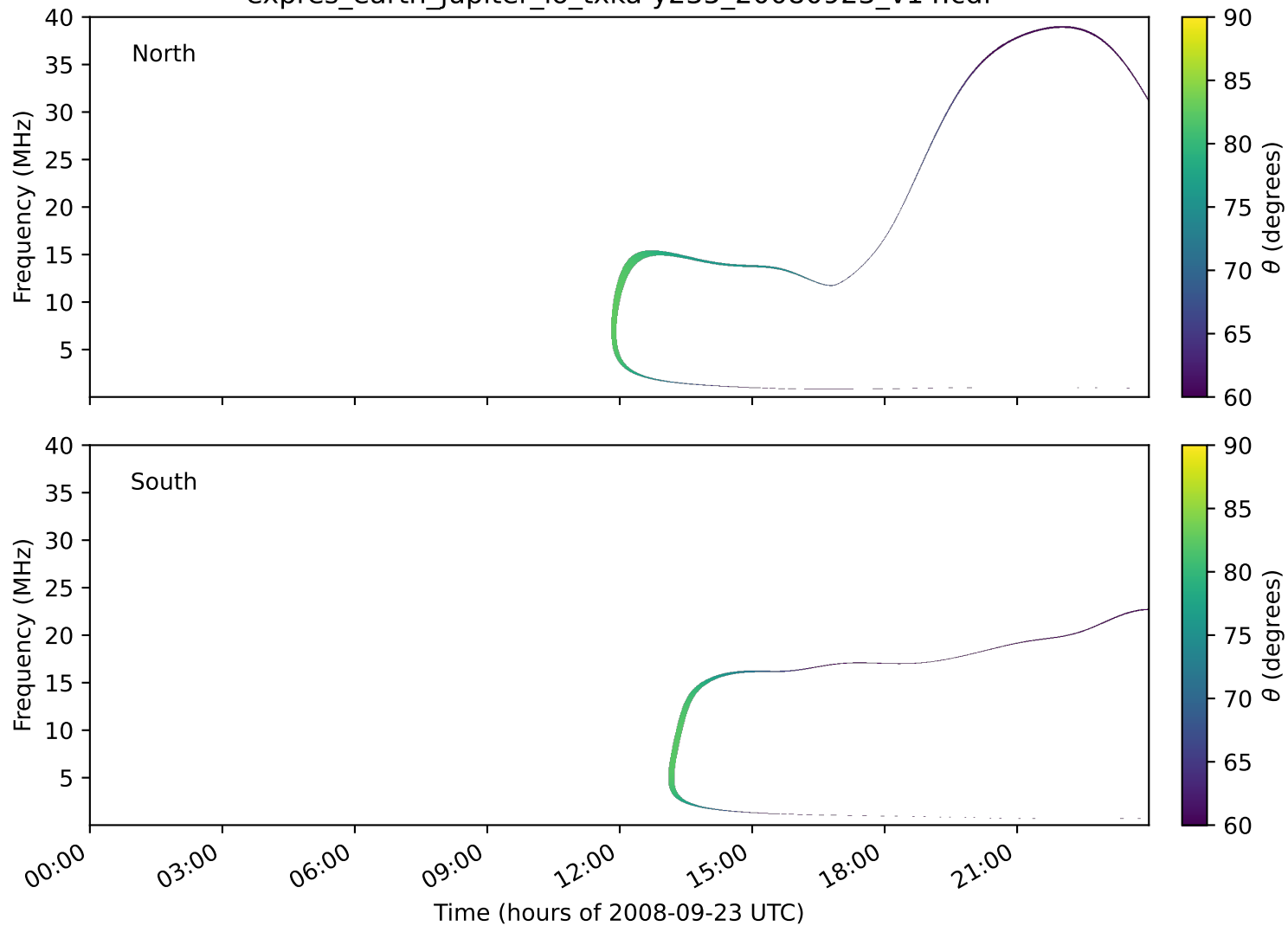
expres_earth_jupiter_io_txka-y235_20080923_v14.cdf
