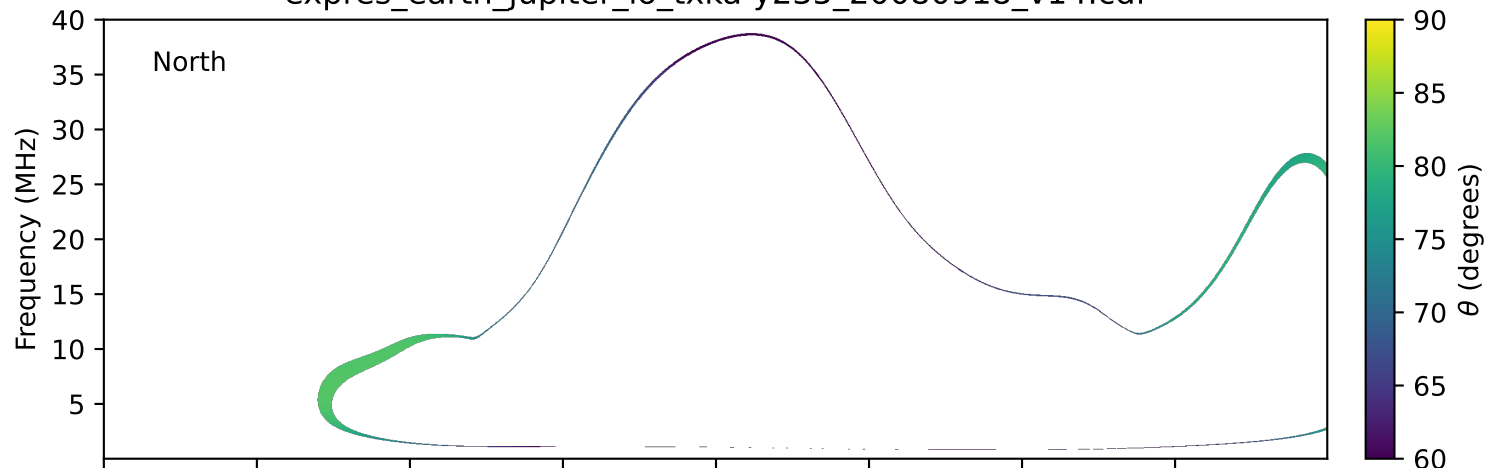
expres_earth_jupiter_io_txka-y235_20080918_v14.cdf
