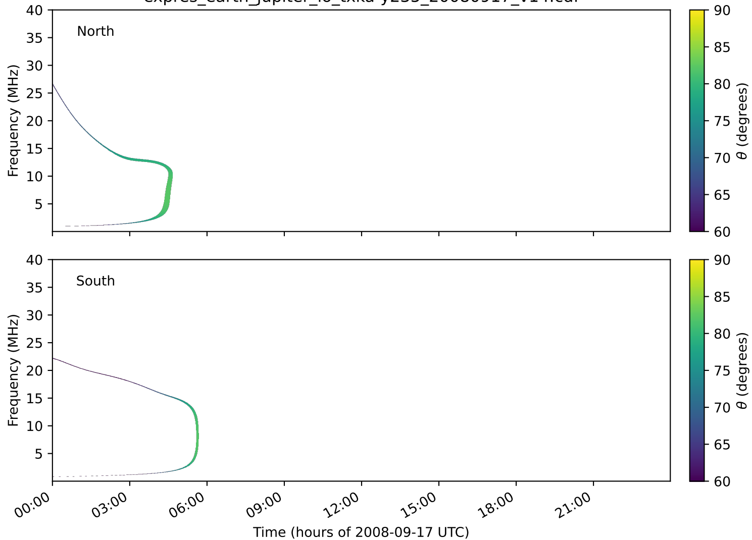
expres_earth_jupiter_io_txka-y235_20080917_v14.cdf
