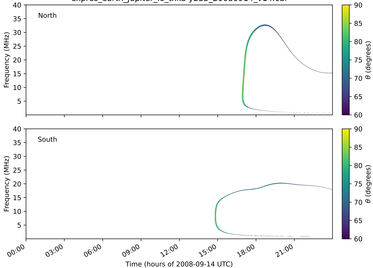
expres_earth_jupiter_io_txka-y235_20080914_v14.cdf
