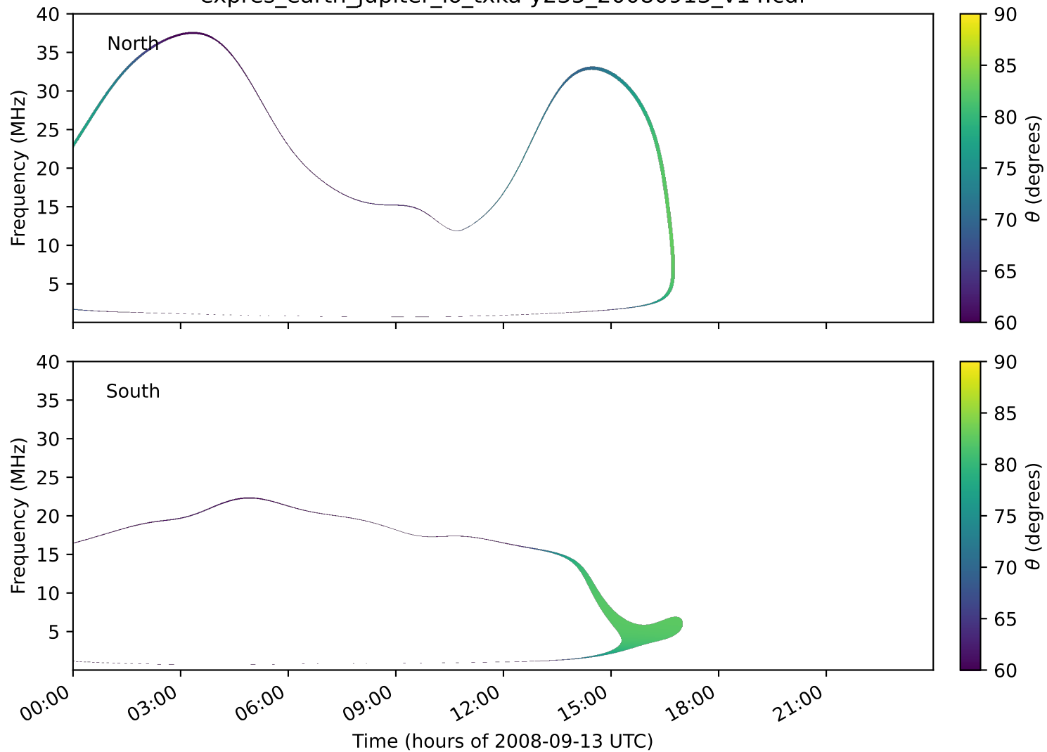
expres_earth_jupiter_io_txka-y235_20080913_v14.cdf
