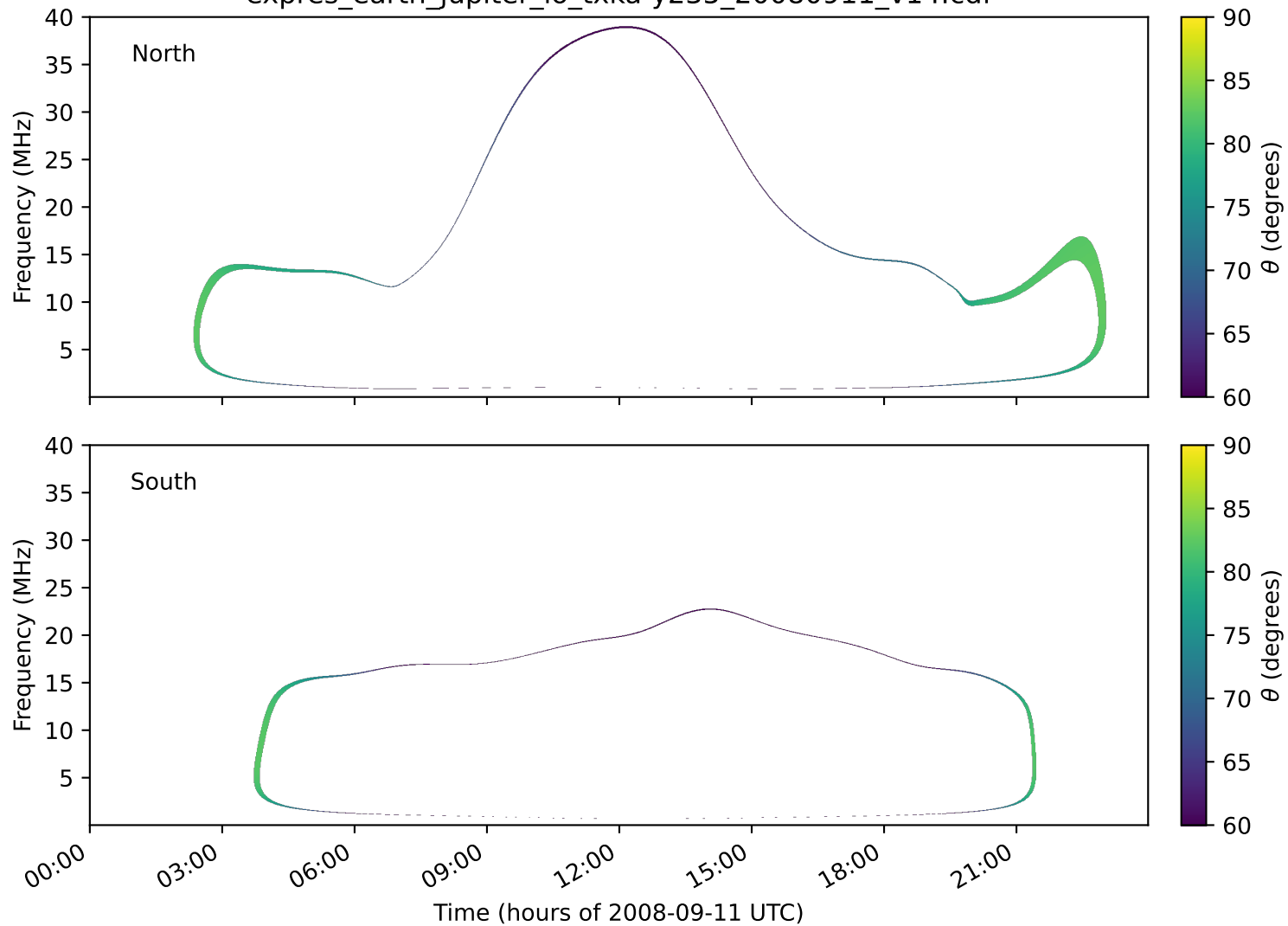
expres_earth_jupiter_io_txka-y235_20080911_v14.cdf
