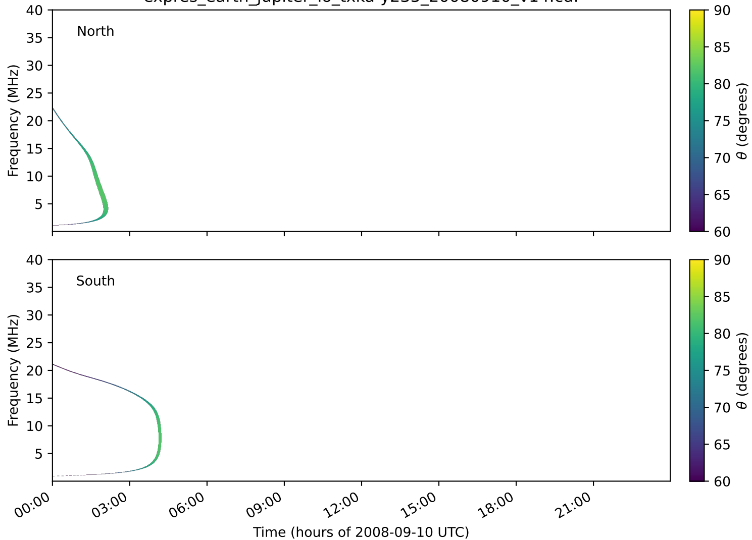
expres_earth_jupiter_io_txka-y235_20080910_v14.cdf
