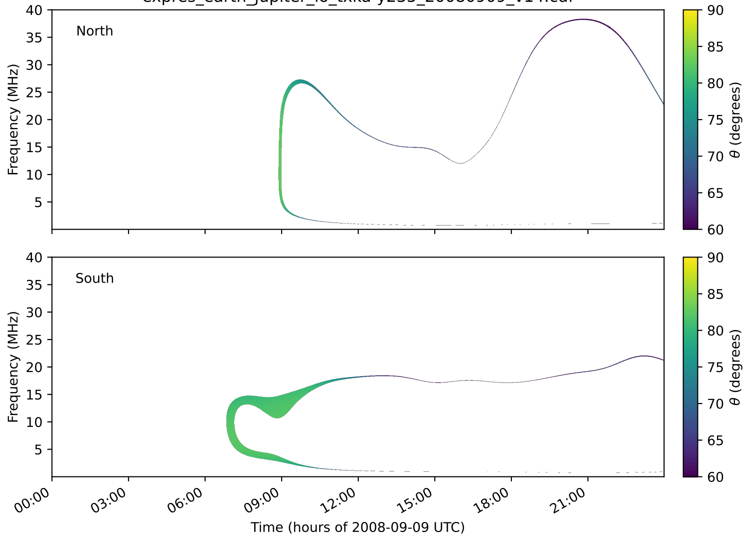
expres_earth_jupiter_io_txka-y235_20080909_v14.cdf
