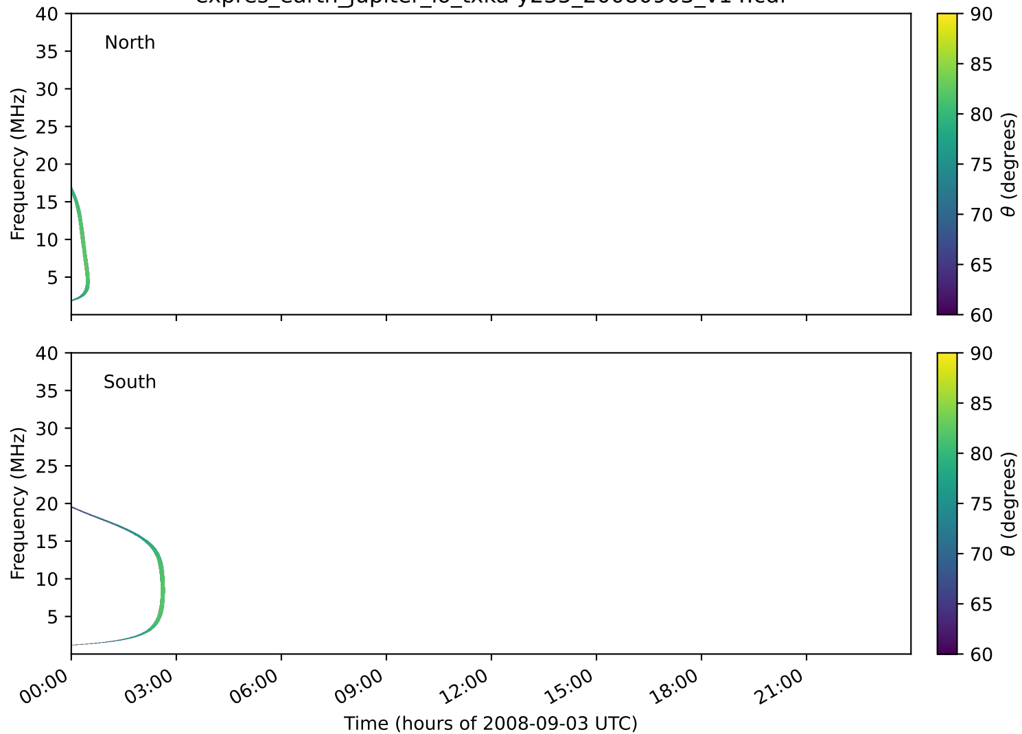
expres_earth_jupiter_io_txka-y235_20080903_v14.cdf
