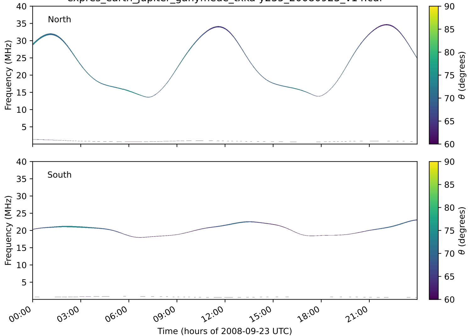
expres_earth_jupiter_ganymede_txka-y235_20080923_v14.cdf
