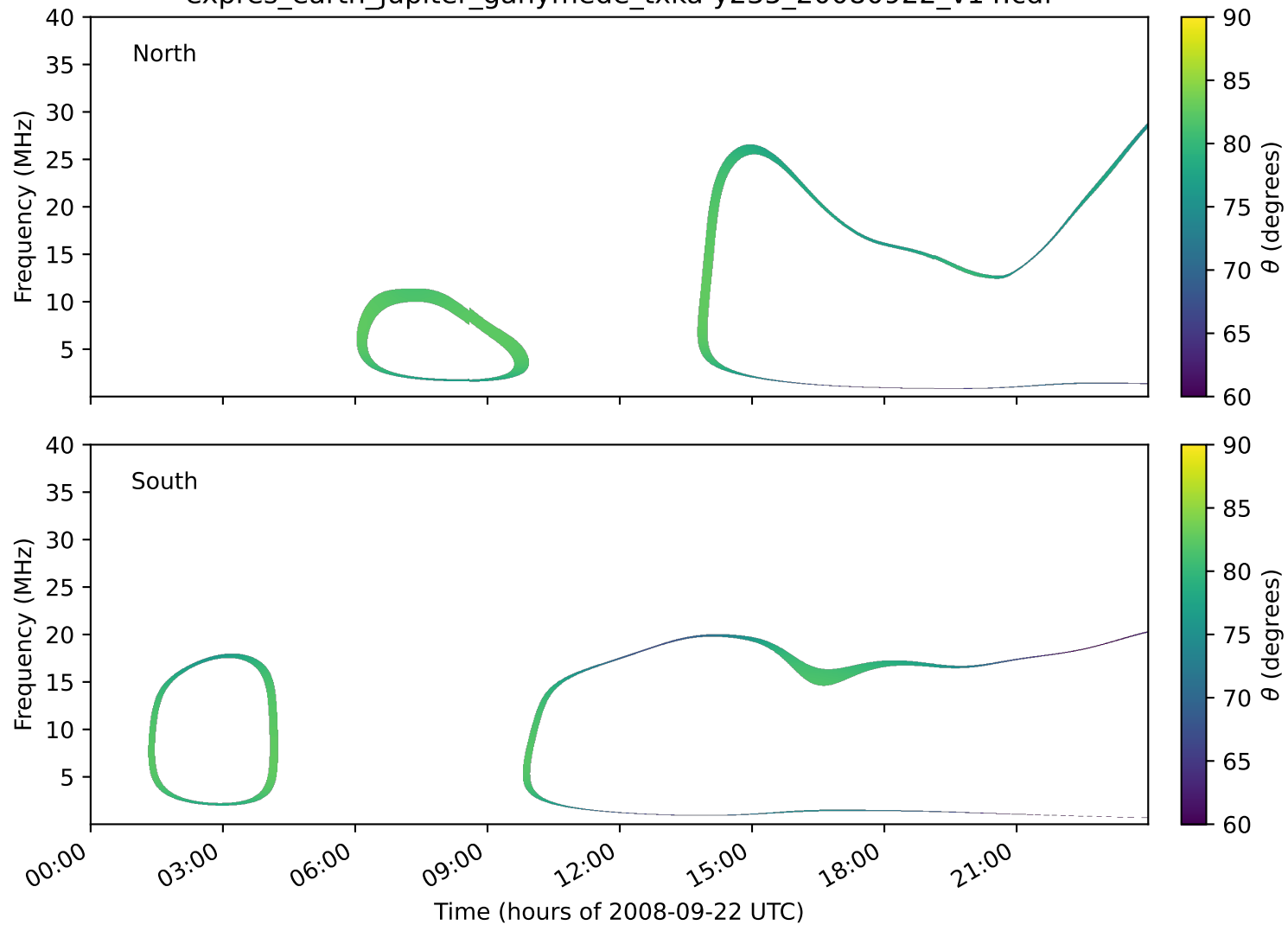
expres_earth_jupiter_ganymede_txka-y235_20080922_v14.cdf
