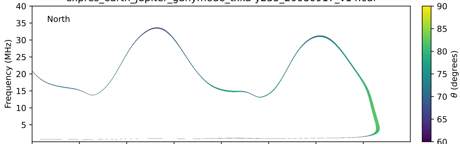
expres_earth_jupiter_ganymede_txka-y235_20080917_v14.cdf
