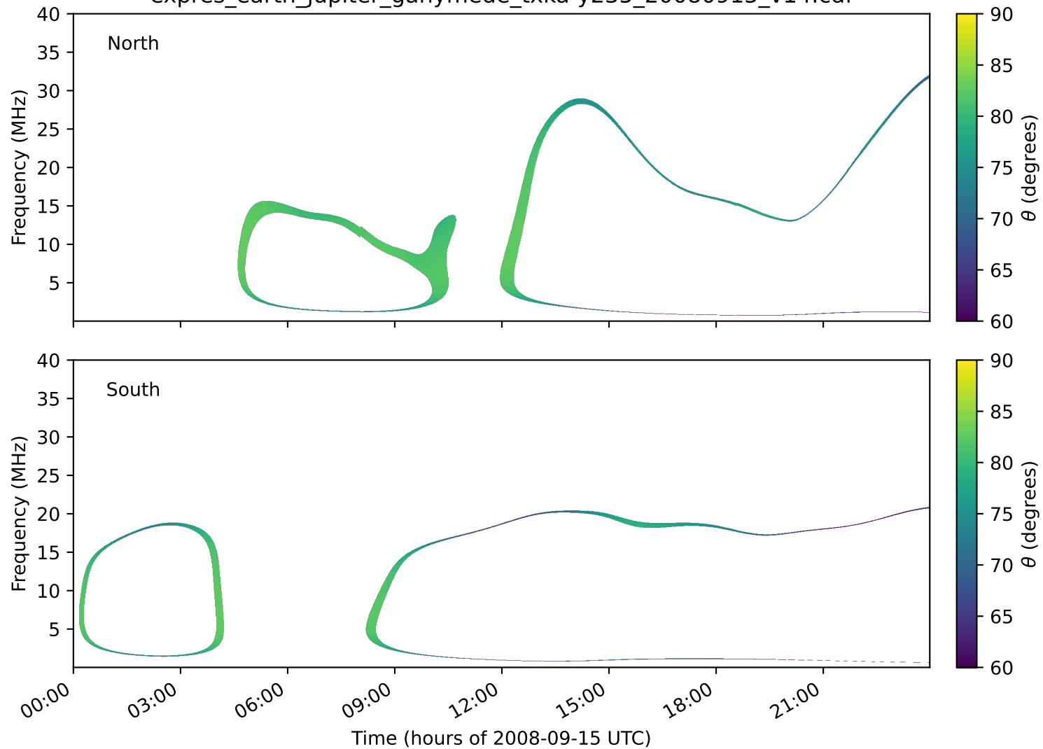
expres_earth_jupiter_ganymede_txka-y235_20080915_v14.cdf
