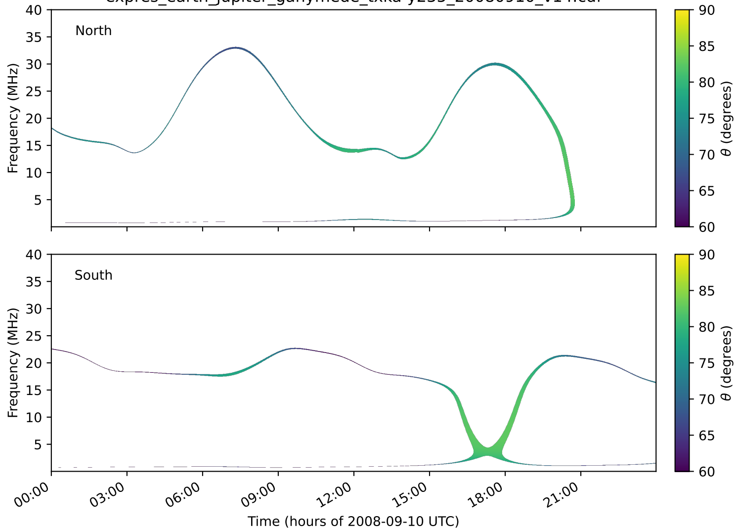
expres_earth_jupiter_ganymede_txka-y235_20080910_v14.cdf
