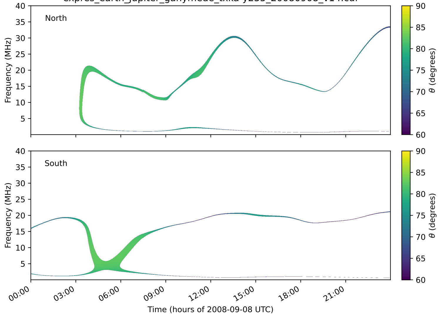
expres_earth_jupiter_ganymede_txka-y235_20080908_v14.cdf
