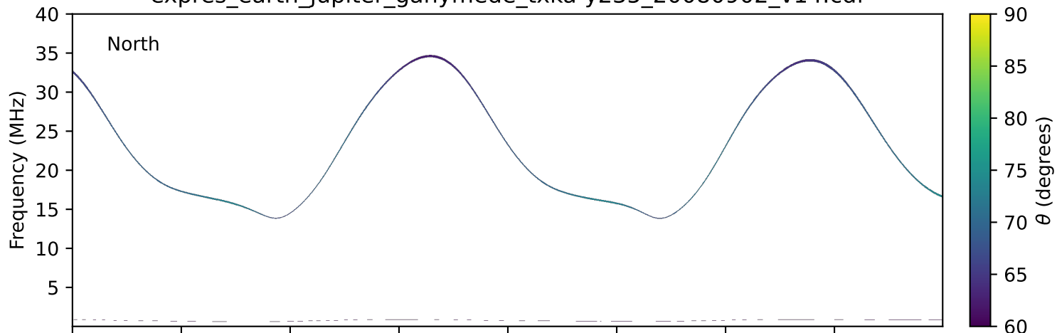
expres_earth_jupiter_ganymede_txka-y235_20080902_v14.cdf
