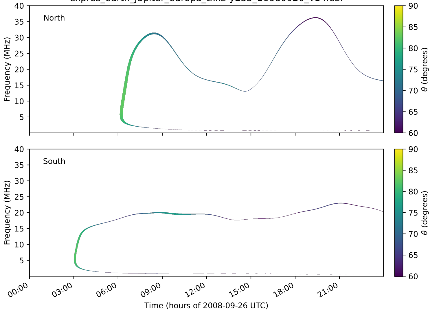
expres_earth_jupiter_europa_txka-y235_20080926_v14.cdf
