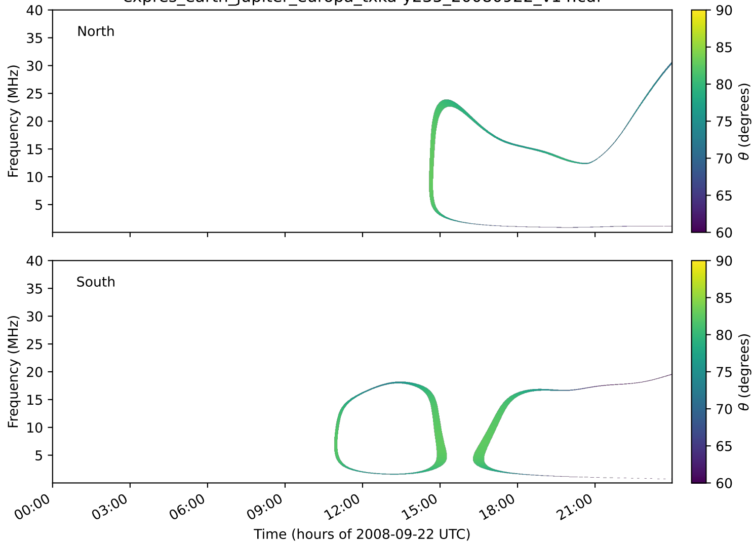
expres_earth_jupiter_europa_txka-y235_20080922_v14.cdf
