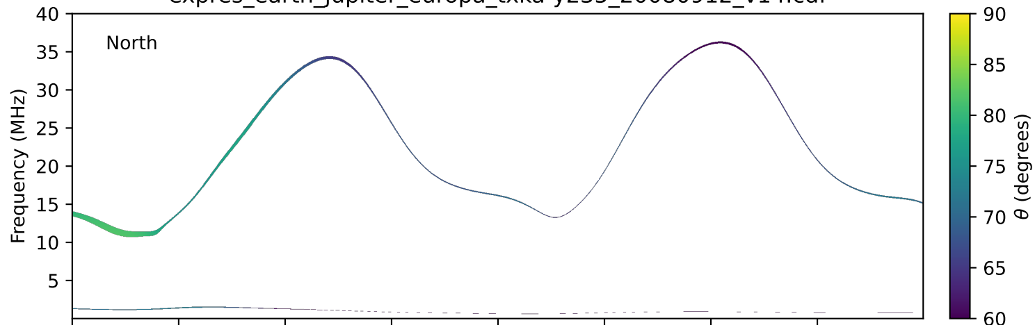
expres_earth_jupiter_europa_txka-y235_20080912_v14.cdf
