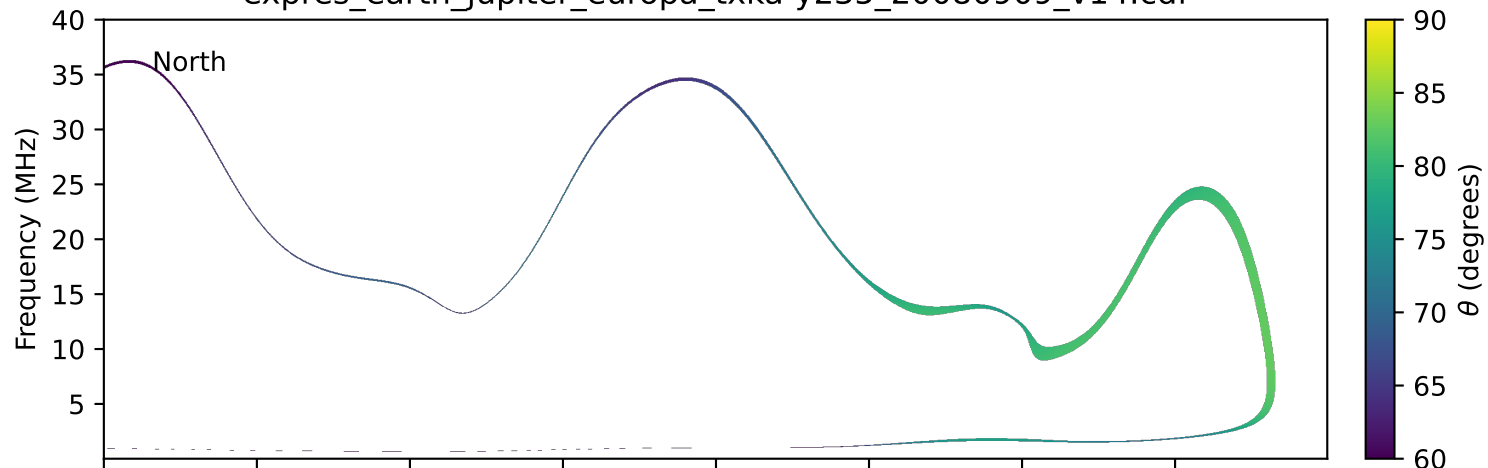
expres_earth_jupiter_europa_txka-y235_20080909_v14.cdf
