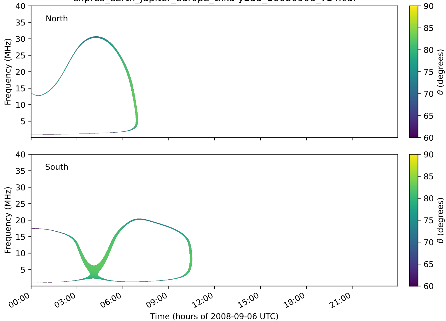
expres_earth_jupiter_europa_txka-y235_20080906_v14.cdf
