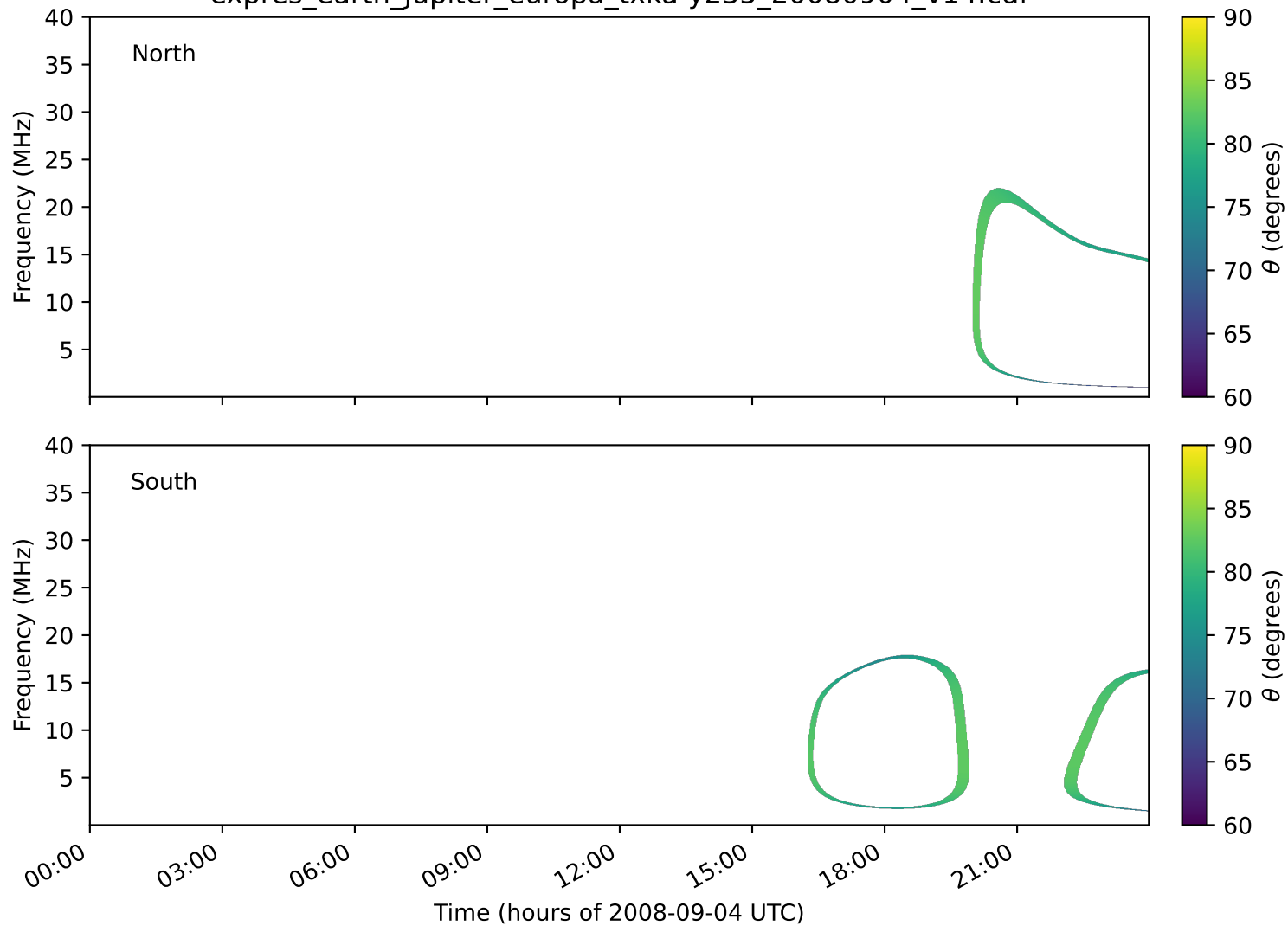
expres_earth_jupiter_europa_txka-y235_20080904_v14.cdf
