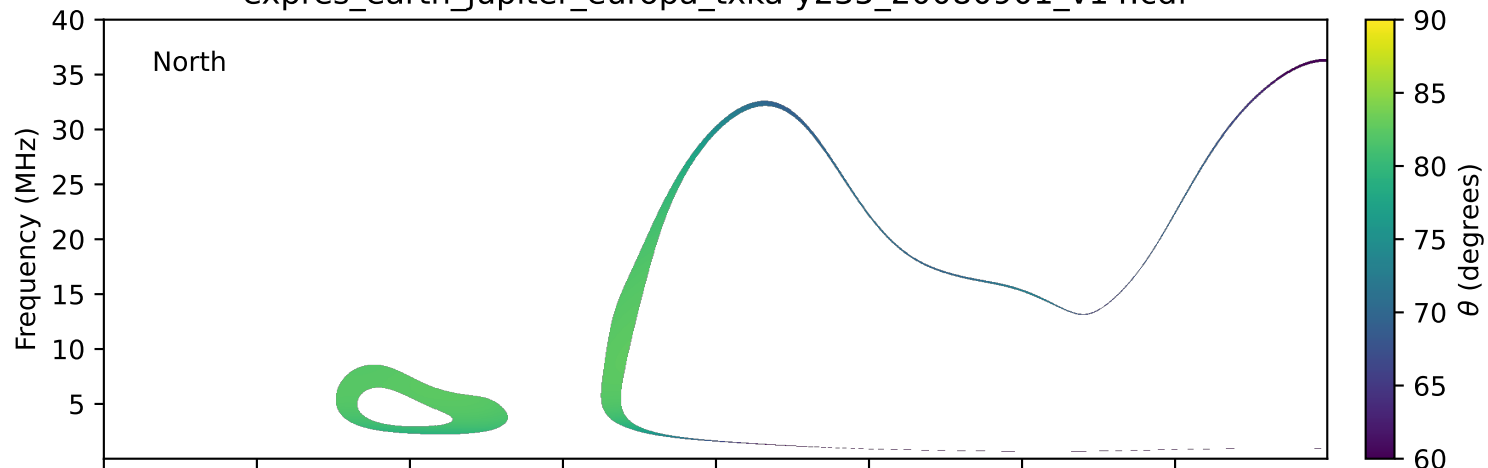
expres_earth_jupiter_europa_txka-y235_20080901_v14.cdf
