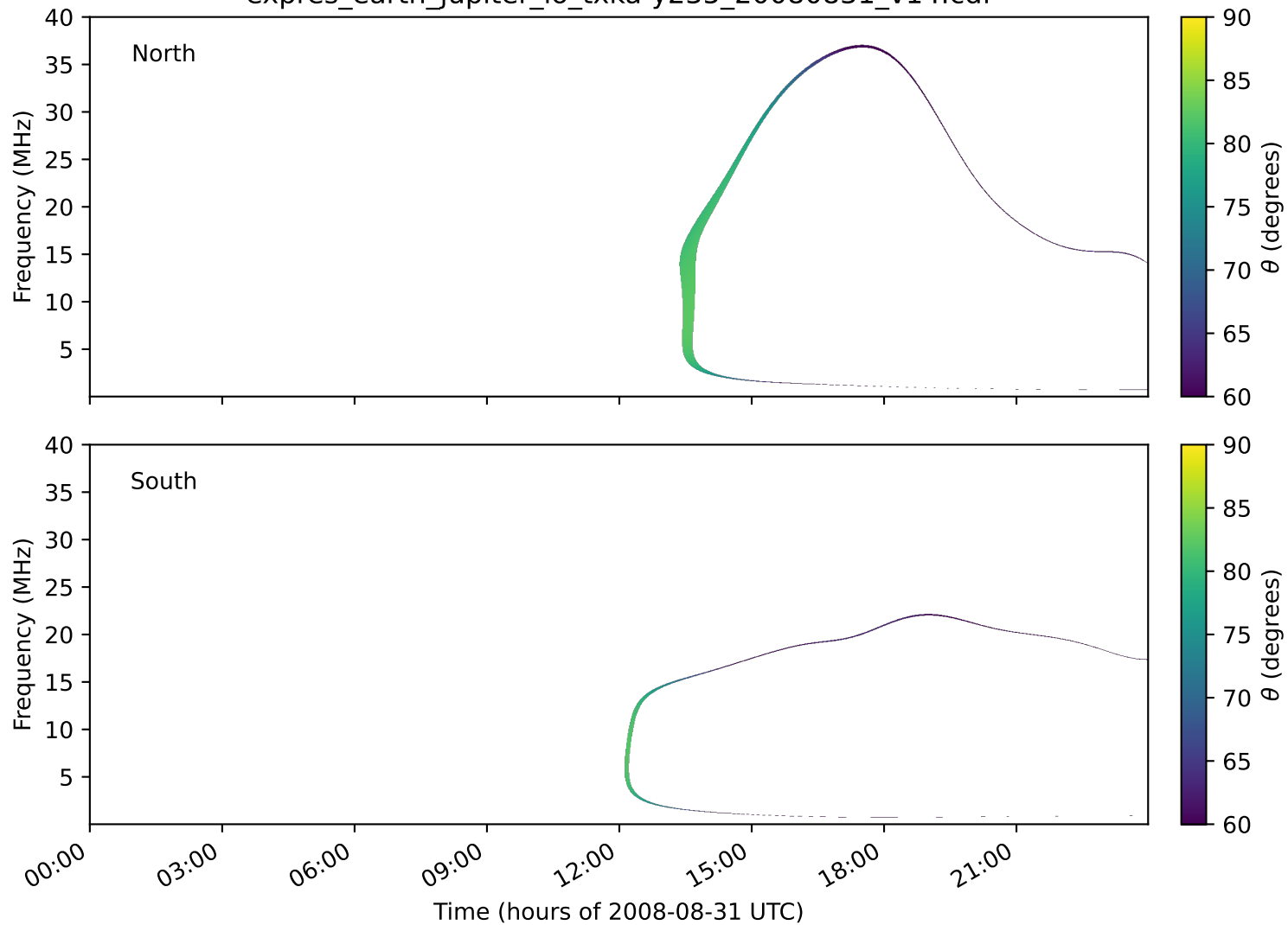
expres_earth_jupiter_io_txka-y235_20080831_v14.cdf
