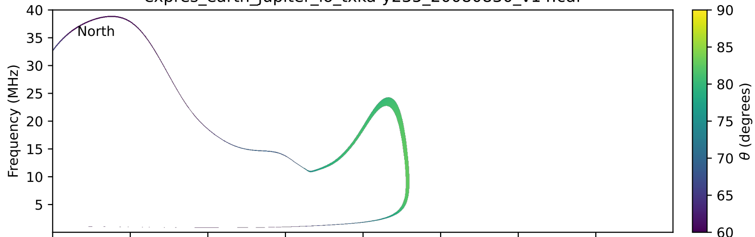
expres_earth_jupiter_io_txka-y235_20080830_v14.cdf
