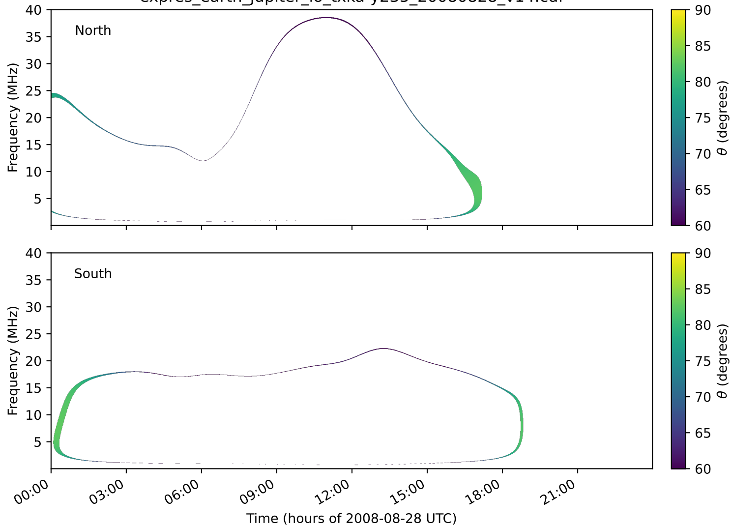
expres_earth_jupiter_io_txka-y235_20080828_v14.cdf
