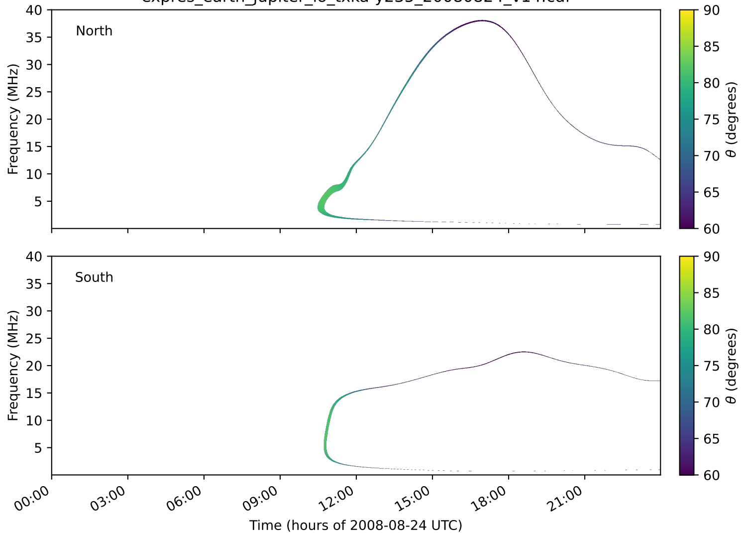
expres_earth_jupiter_io_txka-y235_20080824_v14.cdf
