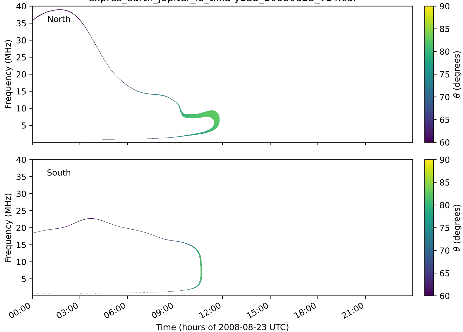
expres_earth_jupiter_io_txka-y235_20080823_v14.cdf
