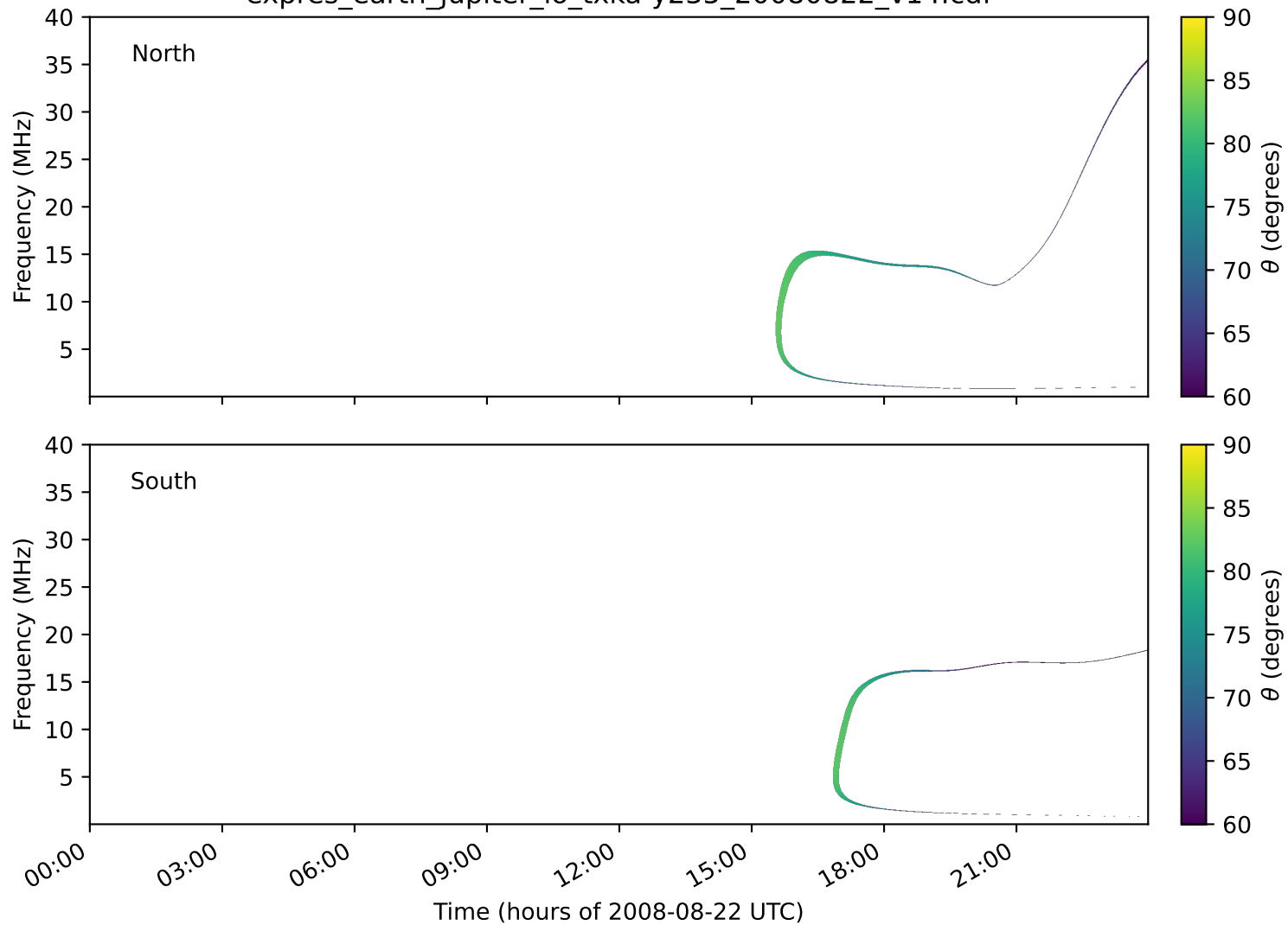
expres_earth_jupiter_io_txka-y235_20080822_v14.cdf
