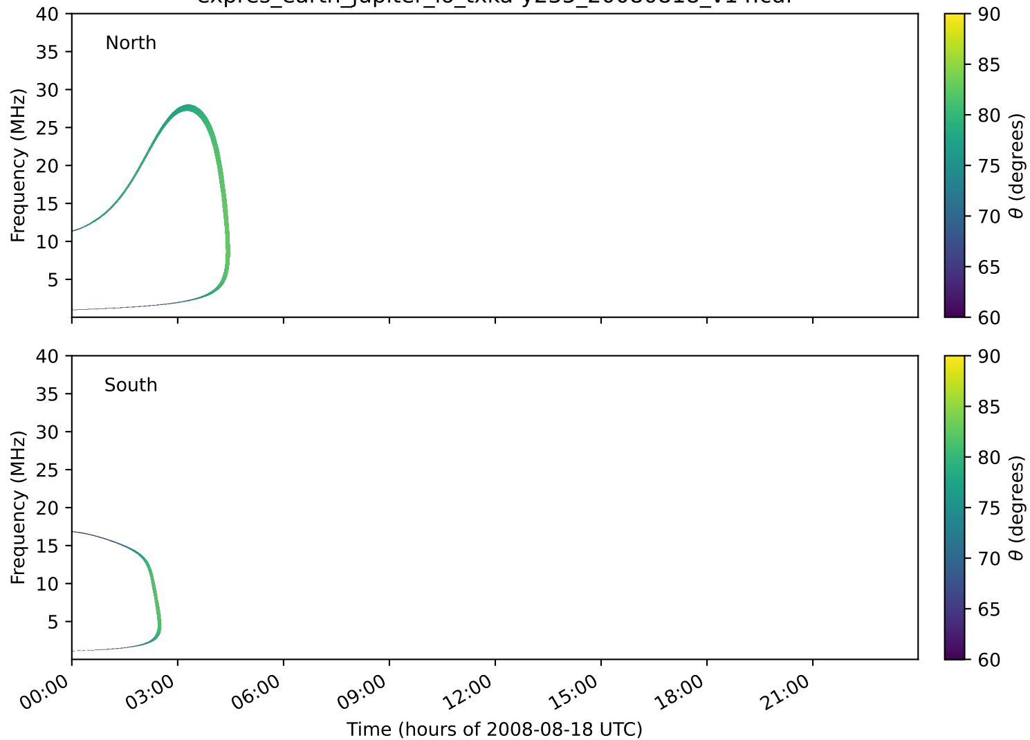
expres_earth_jupiter_io_txka-y235_20080818_v14.cdf
