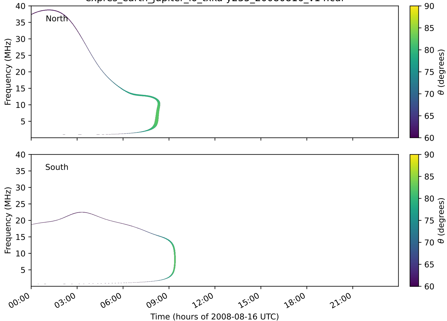
expres_earth_jupiter_io_txka-y235_20080816_v14.cdf
