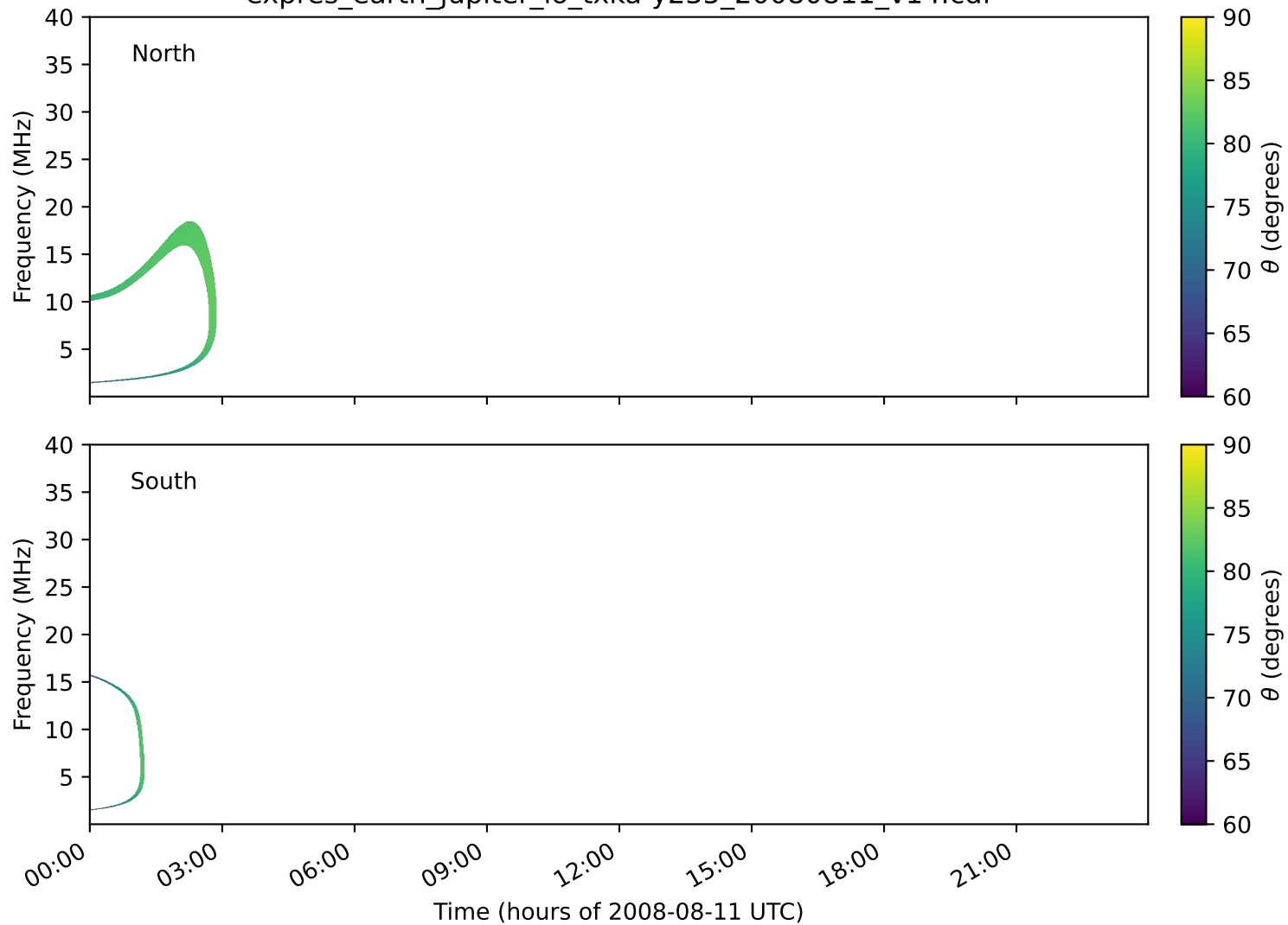
expres_earth_jupiter_io_txka-y235_20080811_v14.cdf
