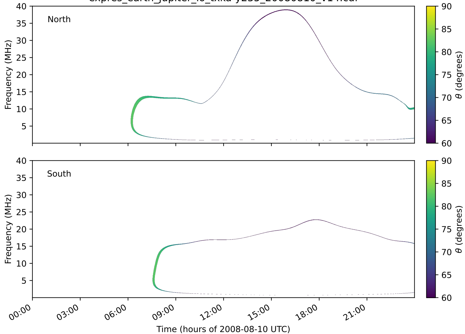
expres_earth_jupiter_io_txka-y235_20080810_v14.cdf
