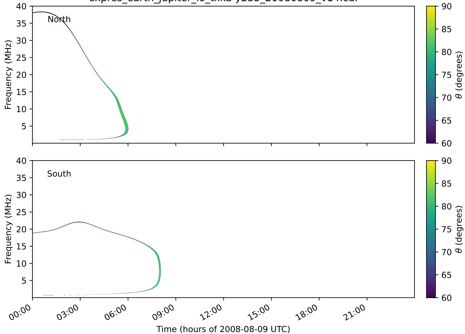
expres_earth_jupiter_io_txka-y235_20080809_v14.cdf
