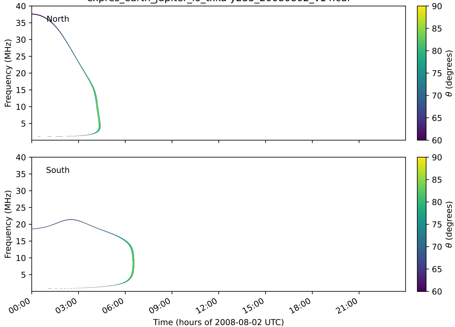
expres_earth_jupiter_io_txka-y235_20080802_v14.cdf
