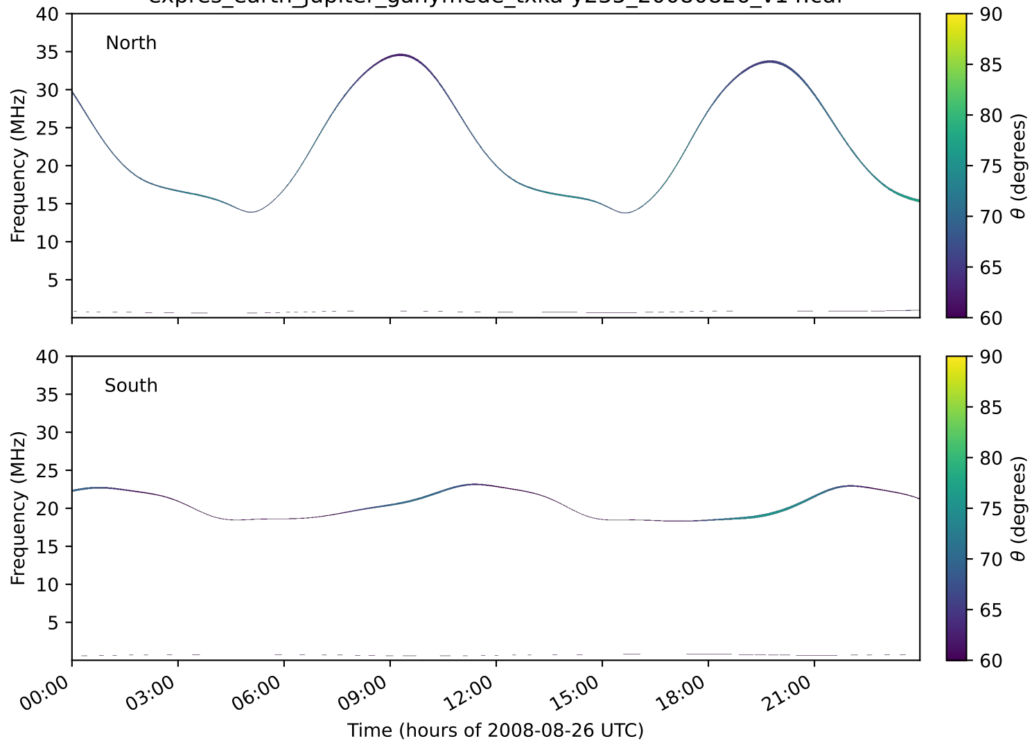
expres_earth_jupiter_ganymede_txka-y235_20080826_v14.cdf
